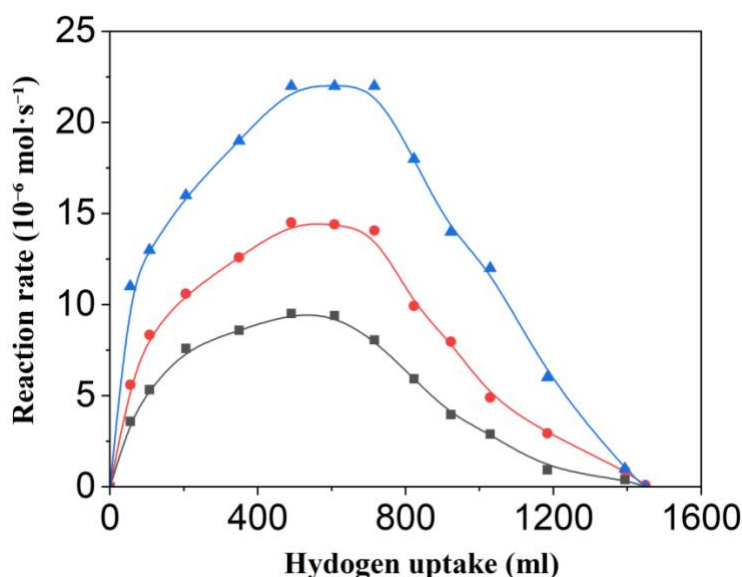
Figure 7. Kinetic curves of benzene hydrogenation over Ru/D catalysts with Ru loadings of 0.5%, 1.0%, and 1.5% at 90 \text{ }^\circ\text{C} .
