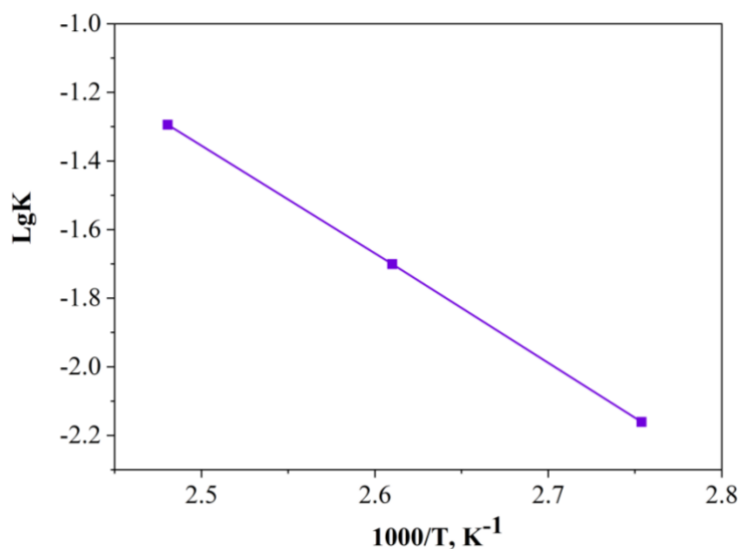
Figure 6. Logarithmic dependence of the rate constant on the reciprocal temperature.
